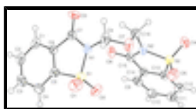
Fig. 1. The title molecule with the displacement ellipsoids plotted at 50% probability level (Farrugia, 1997).
