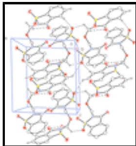
Fig. 2. Unit cell packing of the title compound showing hydrogen bonds by dashed lines; the H-atoms not involved in H-bonds have been excluded for clarity.
